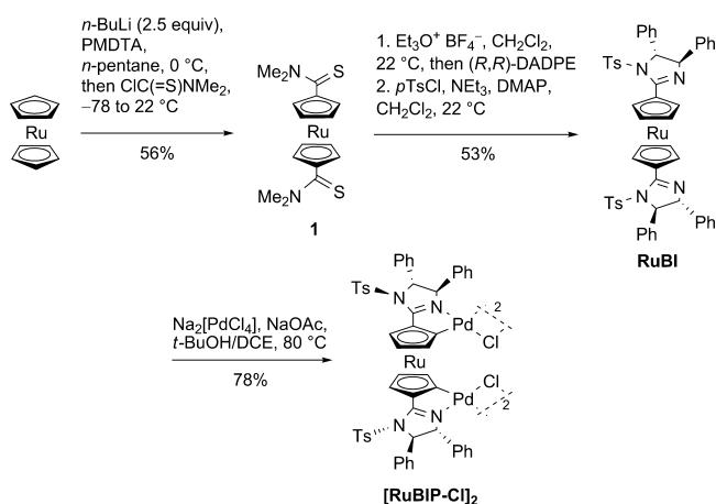
Scheme 1. Diastereoselective Synthesis of the Chloride Bridged Bispalladacycle [RuBIP-Cl] 2
