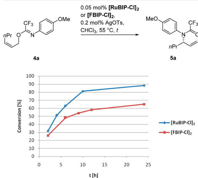
Figure 4. Comparison of the reactivity using the bis-Pd precatalysts [\text{RuBIP-Cl}]_2 (blue curve) and [\text{FBIP-Cl}]_2 (red curve)—activated by AgOTs—for the rearrangement of substrates 4a by monitoring via 1 H NMR (conditions of Table 1, entries 1 and 2).
