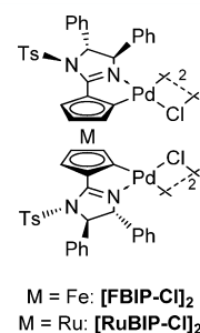
Figure 1. [FBIP-Cl] 2 and [RuBIP-Cl] 2 .
