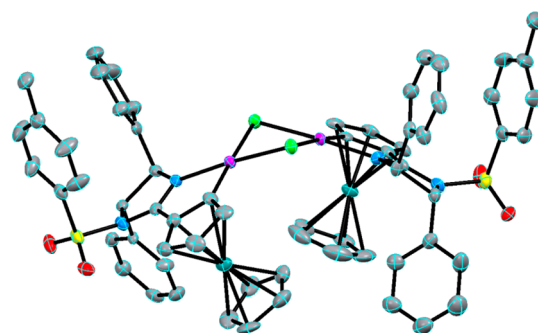
Figure 3. X-ray single crystal structure analysis of [\text{RuIP-Cl}]_2 (color code: C (gray); N (blue); O (red); S (yellow); Cl (green); Ru (turquoise); Pd (magenta)). Hydrogen atoms and dichloromethane (1 per unit cell) are omitted for clarity in the ORTEP plot (ellipsoids at 50% probability level). Selected bond lengths (Å) and angles (deg): C–Pd, 1.959(6)–1.967(5); N–Pd, 2.025(5)–2.042(5); Cl cis-to-C –Pd, 2.3328(14)–2.3348(14); Cl trans-to-C –Pd, 2.4506(13); C–Pd–N, 80.4(2)–80.6(2); C–Pd–Cl cis-to-C , 93.35(18)–94.41(17); N–Pd–Cl trans-to-C , 96.01(13)–97.22(13); Cl–Pd–Cl, 88.87(5)–88.92(5); N–Pd–Cl cis-to-C , 173.59(13)–173.64(13); C–Pd–Cl trans-to-C , 174.87(16)–176.02(17).
