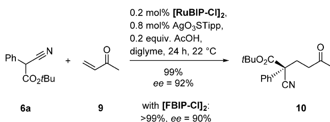
Scheme 4. Comparison of RuBIP and FBIP in the Direct 1,4-Addition of \alpha -Cyanoacetate 6a to MVK
