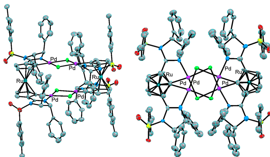
Figure 2. X-ray single crystal structure analysis of [\text{RuBIP-Cl}]_2 (color code: C (gray); N (blue); O (red); S (yellow); Cl (green); Ru (turquoise); Pd (magenta)). Hydrogen atoms and chloroform (7 per unit cell) are omitted for clarity in the ORTEP plot (ellipsoids at 50% probability level). Two different views are shown. Selected bond lengths (Å) and angles (deg): C–Pd, 1.914(16)–2.00(2); N–Pd, 1.977(17)–2.075(16); Cl cis-to-C –Pd, 2.309(5)–2.329(5); Cl trans-to-C –Pd, 2.428(5)–2.443(5); C–Pd–N, 78.7(8)–83.1(7); C–Pd–Cl cis-to-C , 93.1(6)–95.8(6); N–Pd–Cl trans-to-C , 93.3(4)–95.5(4); Cl–Pd–Cl, 90.48(17)–90.97(16); N–Pd–Cl cis-to-C , 173.0(5)–175.0(4); C–Pd–Cl trans-to-C , 172.9(6)–176.2(6).
